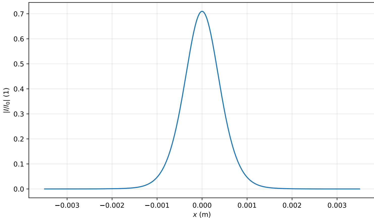
Intensity profile I(x, y = 0, z = 2.866m)/I_0 , P_{in}=0.6P_{cr} , artificial time
